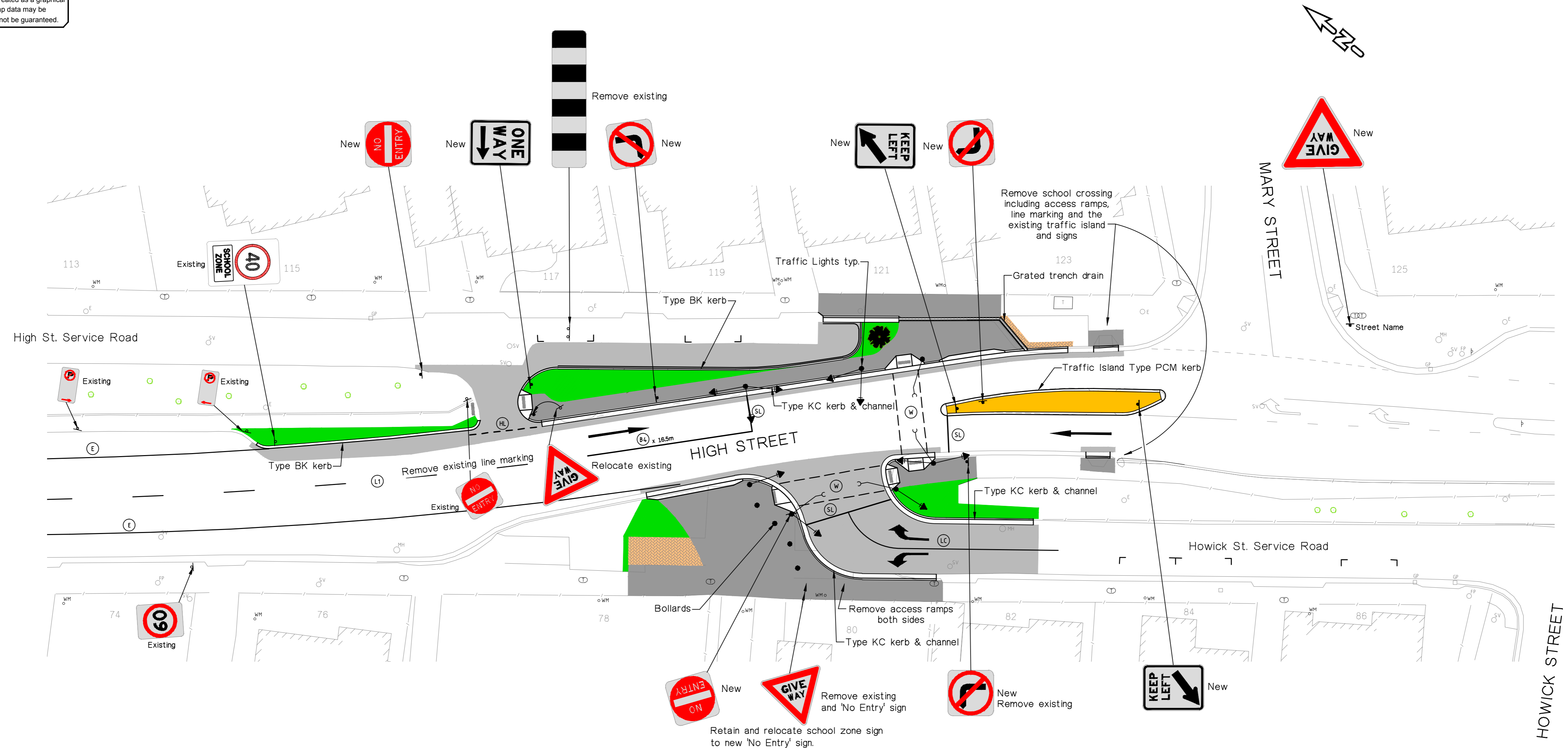
CONCEPT PLAN 1: 250
