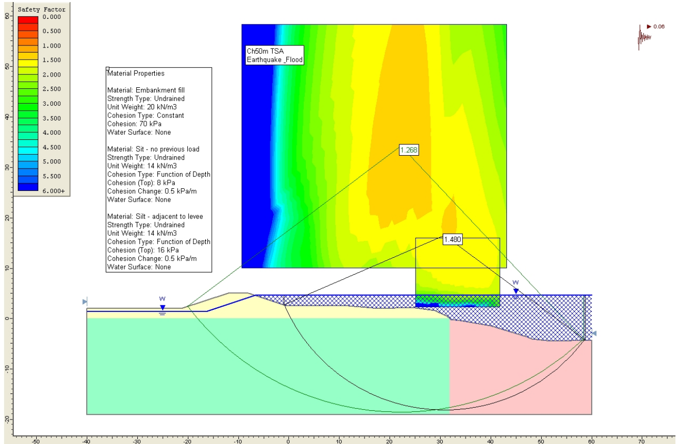
Deep Silt Model 3. Earth levee, no effect of consolidation and river in flood
