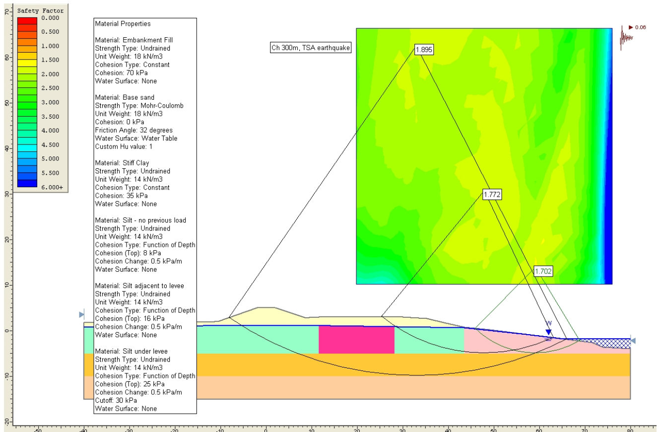
Shallow Silt Model 2. Earth levee, no effect of consolidation
