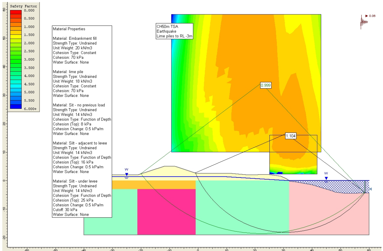
Deep Silt Model 5. Earth levee, strength increase under levee and lime piles to RL -3m
