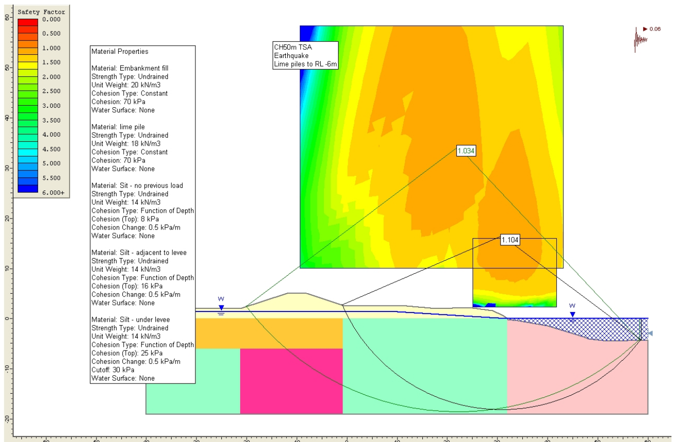
Deep Silt Model 6. Earth levee, strength increase under levee and lime piles to RL -6m
