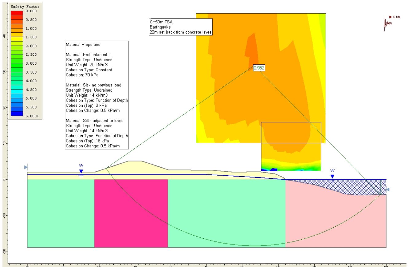
Deep Silt Model 4. Earth levee, strength increase under levee
