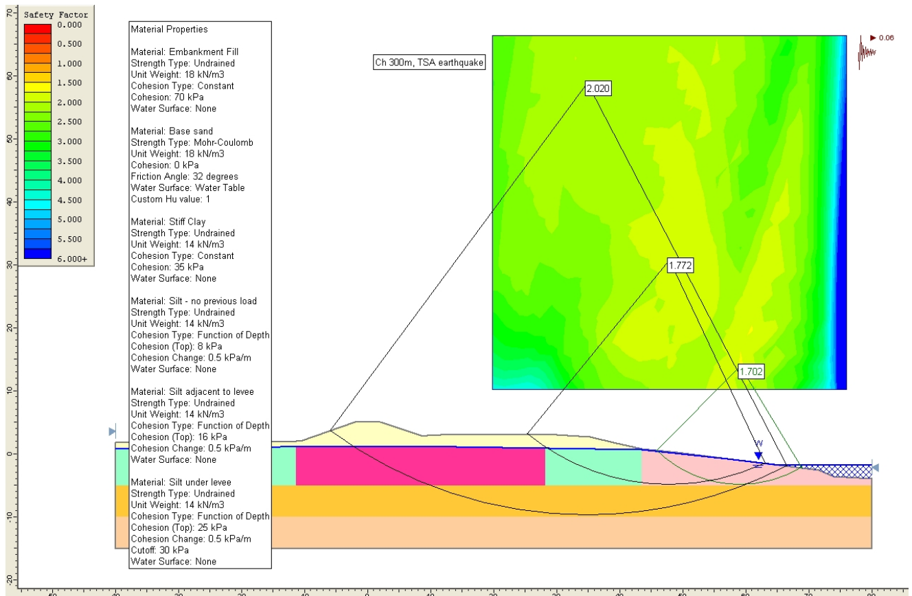
Shallow Silt Model 4. Earth levee, strength increase under levee
