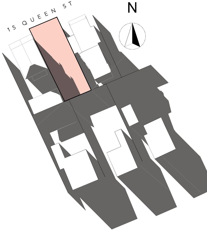
SHADOW STUDY EXISTING JUNE 21 03:30 PM SCALE: 1:500
